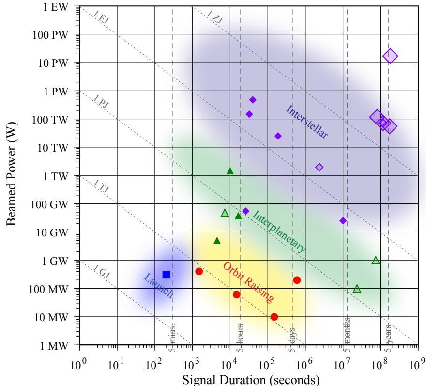
Figure 1. Domains of beam power and radiation duration of power beaming applications shown as squares (launch), circle (orbit raising), triangles (interplanetary) and diamonds (interstellar). Data for the points can be found in the references. The solid points are for radio beaming, while the hollow points indicate visible/near-IR laser beams. For interstellar applications, the point size reflects the velocity, varying from 0.1c to 0.5c .
